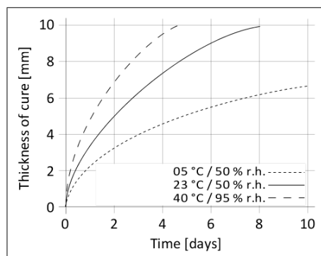
Diagram 1: Curing speed Sikasil® WS-305 KR
