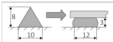
Figure 1: Recommended bead configuration
