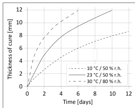
Diagram 1: Curing speed SikaTack® Panel
