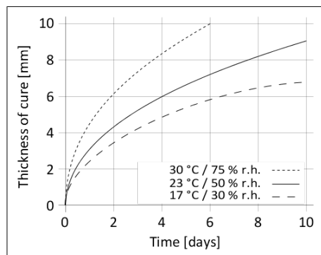
Diagram 1: Curing speed Sikaflex®-215
