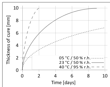
Diagram 1: Curing speed Sikasil® WS-300 KR
