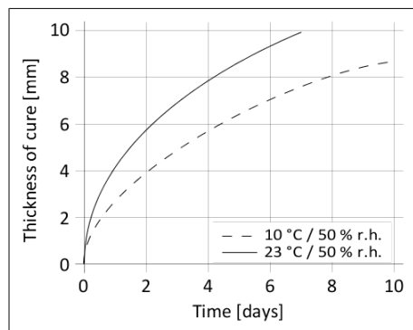
Diagram 1: Curing speed SikaTack® DRIVE (60 min)
